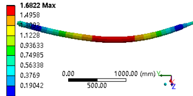
C: Static Structural 静应力51MPa Stress Intensity: 5 Type: Stress Intensity Unit: MPa Time: 2
